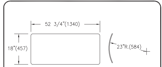
A~ATA54 Buck Dimensions
